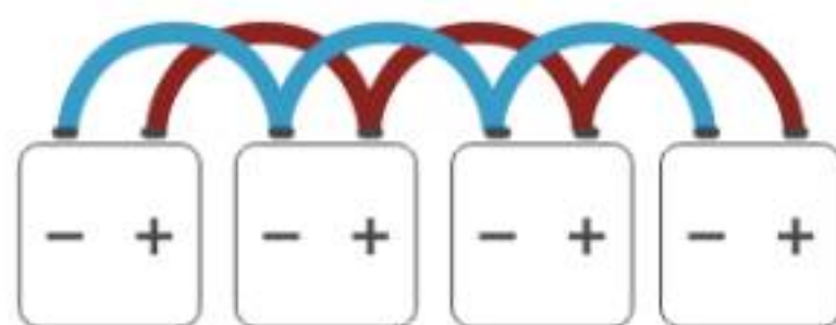
12V(12.8V) 400Ah battery system
